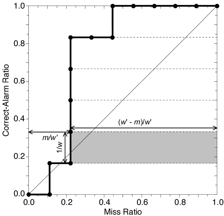
Figure 4. An example ROL diagram for a forecast system with continuous predictand. The example is based on the data in Table 5. Dotted horizontal lines mark the contribution of each hit to the ROL area, and the contribution of the second hit is shaded. The bullets indicate individual points on the ROL curve. See text for further details.
